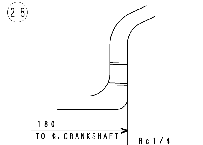
DETAIL OF AIR PRESS. GAUGE ADAPTER
