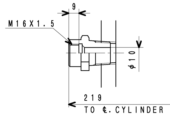
DETAIL OF THERMOMETER & THERMOSWITCH ADAPTER
